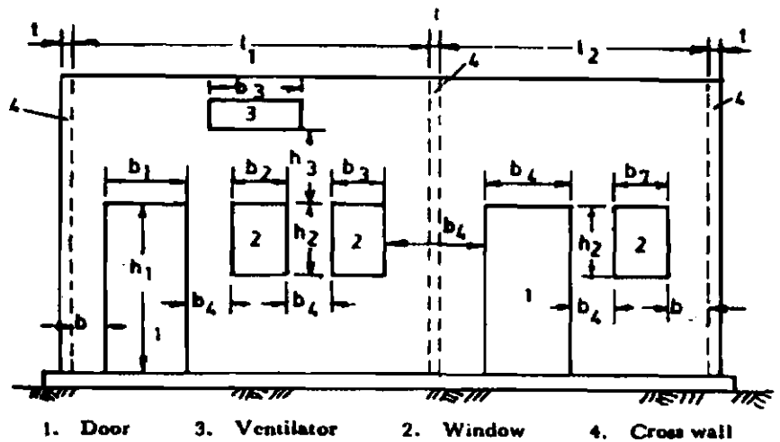
Fig.3:-Opening sizes as per IS: 4326 - 1993
