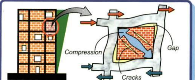
Figure 3: Infill walls move together with the columns under earthquake shaking.
