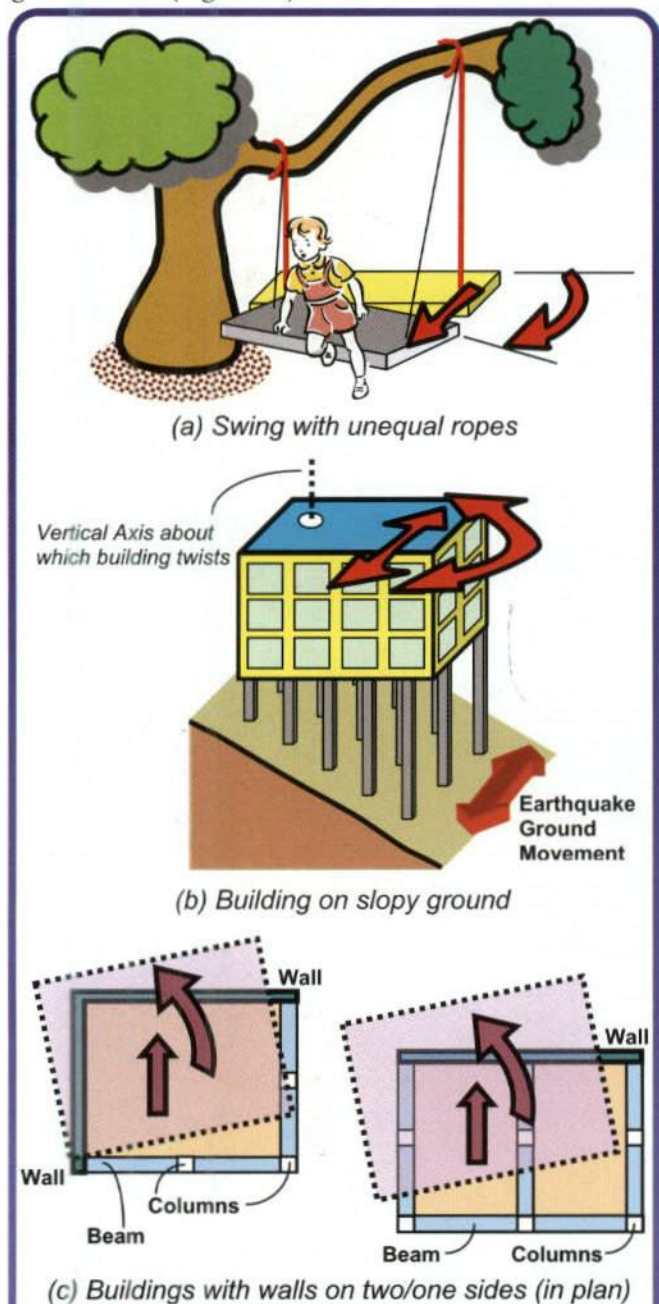
Figure 4: Buildings have unequal vertical members; they cause the building to twist about a vertical axis.
