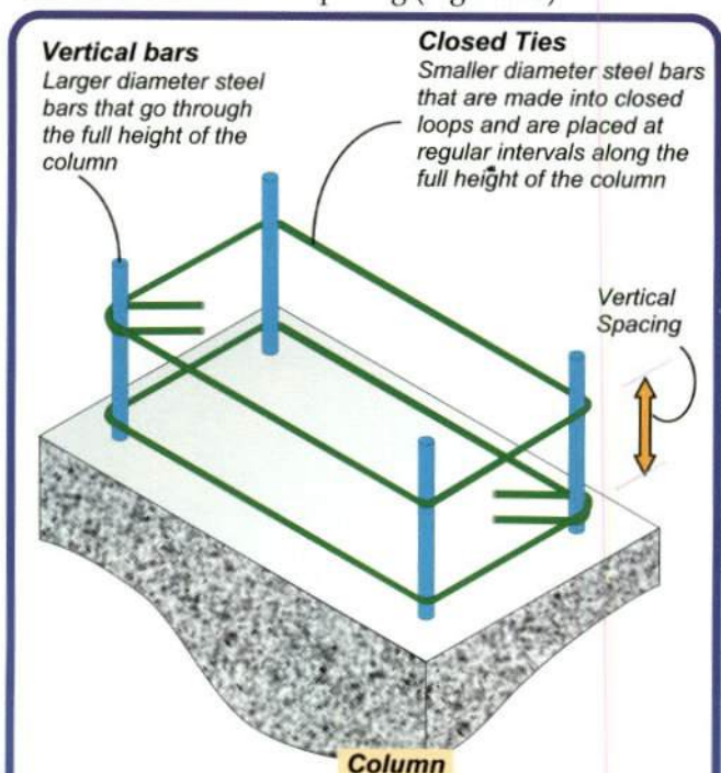
Figure 1: Steel reinforcement in columns – closed ties at close spacing improve the performance of columns under strong earthquake shaking.
