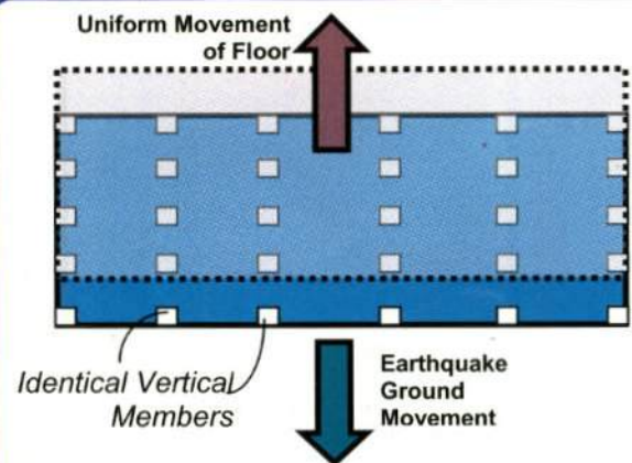
Figure 2: Identical vertical members placed uniformly in plan of building cause all points on the floor to move by same amount.
