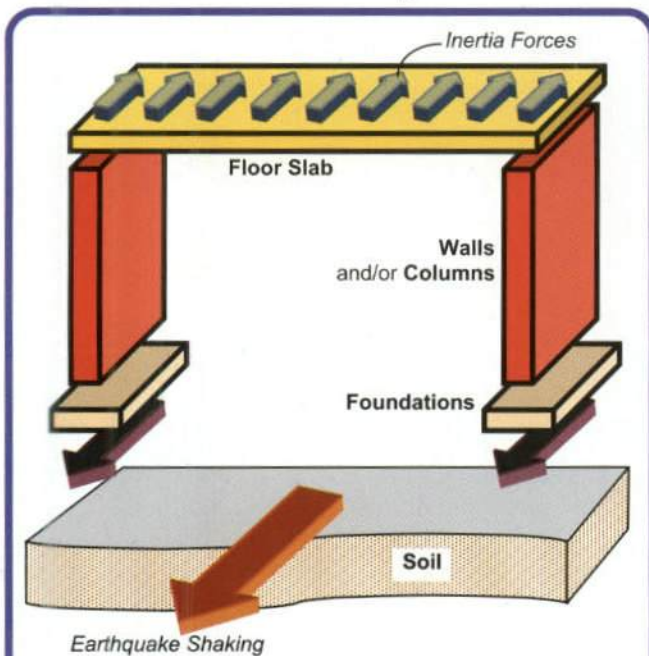
Figure 4: Flow of seismic inertia forces through all structural components.
