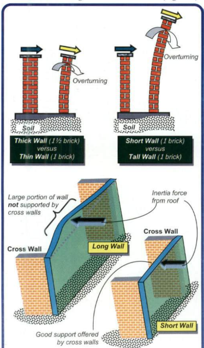
Figure 3: Slender walls are vulnerable – height and length to be kept within limits. Note: In this figure, the effect of roof on walls is not shown.
