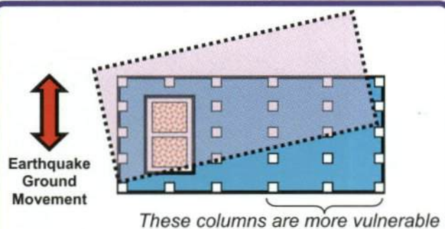
Figure 6: Vertical members of buildings that move more horizontally sustain more damage.
