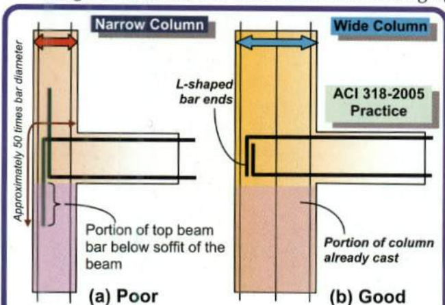
Figure 5: Anchorage of beam bars in exterior joints – diagrams show elevation of joint region.
