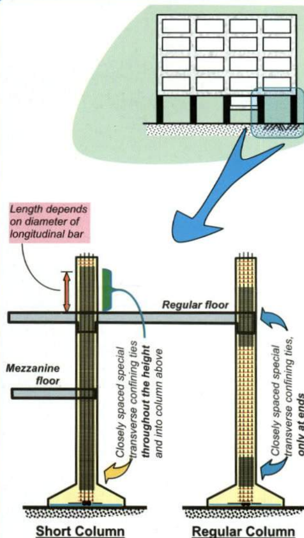
Figure 5: Details of reinforcement in a building with short column effect in some columns – additional special requirements are given in IS:13920-1993 for the short columns.
