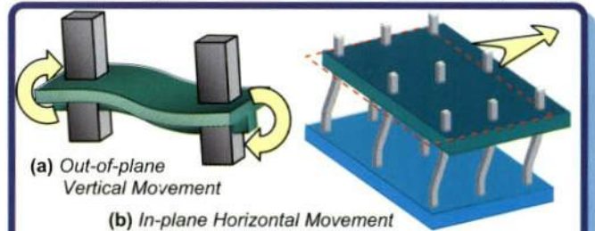
Figure 2: Floor bends with the beam but moves all columns at that level together.
