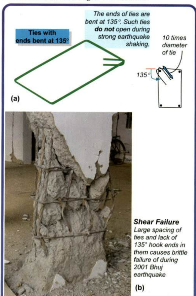
Figure 2: Steel reinforcement in seismic columns – closed ties with 135° hooks are required as per Indian Ductile Detailing Code IS:13920-1993.
