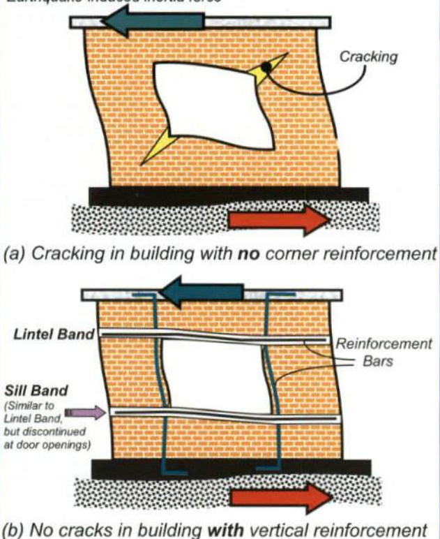
Figure 5: Cracks at corners of openings in a masonry building – reinforcement around them helps.
