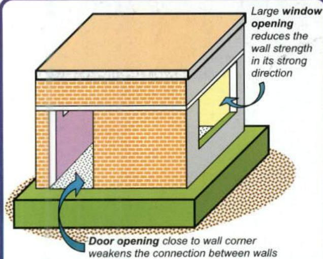
Figure 3: Openings weaken walls in a masonry building – a single closed horizontal band must be provided above all of them.
